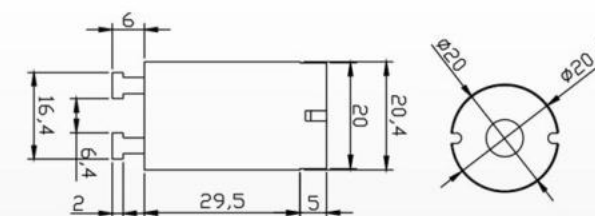
S-2 Material: PP Packing: 1000pcs/ctn G.W: 4.7kgs Ctn Size: 44X23X22cm
