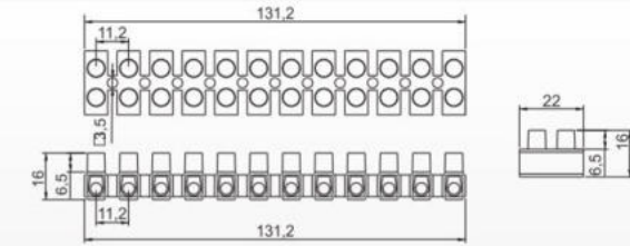
H-16B(H-16A 12mm 2 )
