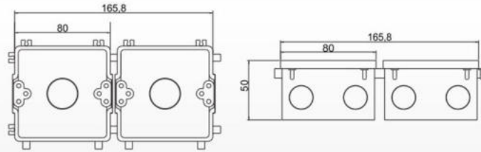
HS-80X80X50 Material:PVC
