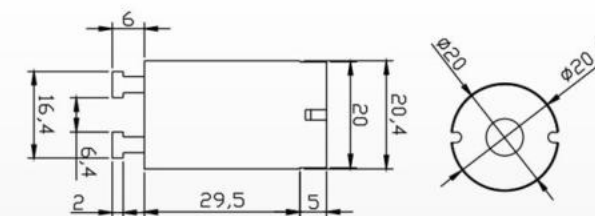
S-5 Material: PP Packing: 1000pcs/ctn G.W: 4.7kgs Ctn Size: 44X23X22cm
