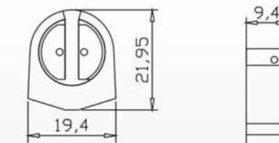
HD-2C(G5) Material: PC Packing:5000pcs/ctn G.W:12.1kgs Ctn Size: 38X28X30cm
