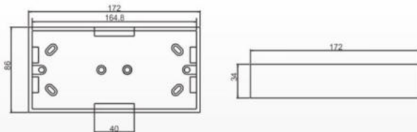
HS-2P Material:PVC
