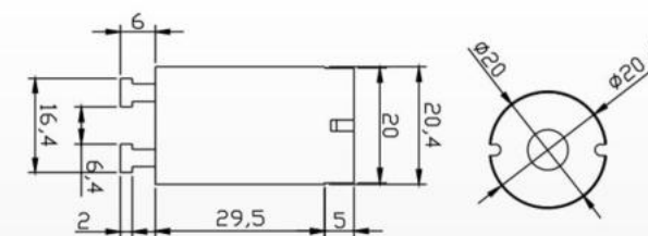
S-6 Material: PP Packing: 1000pcs/ctn G.W: 4.7kgs Ctn Size: 44X23X22cm
