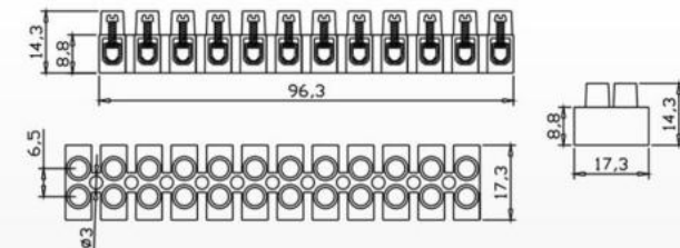
JP-PA7-FDS(12P) (17.5A,450V) Flat Base,With Spring Material: PA,Steel Insert
