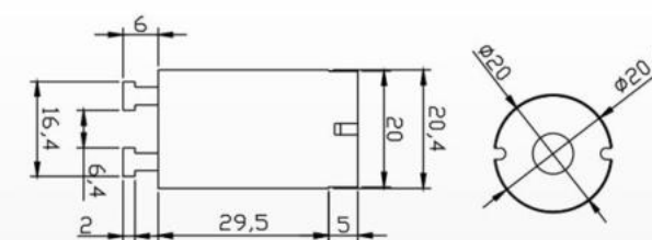
S-1 Material: PP Packing: 1000pcs/ctn G.W: 4.7kgs Ctn Size: 44X23X22cm
