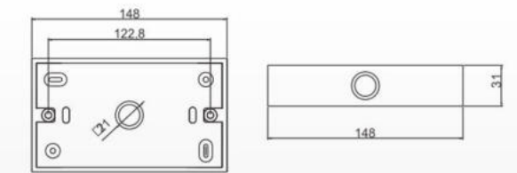
HS-36(148x86x31mm) Material:PVC
