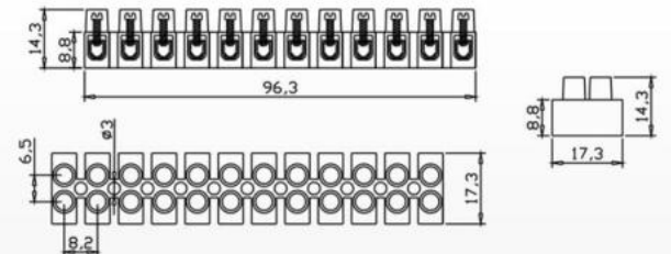
JP-PA7-H(12P) (17.5A,450V) Highback Material: PA,Steel Insert
