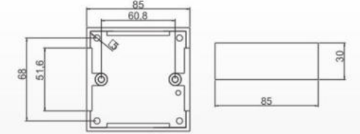
HS-85x85x30 Material:PVC
