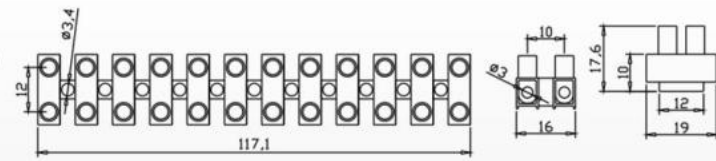
HA-19 (H-5A,6mm 2 )
