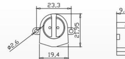
HD-2B(G5) Material: PC Packing:5000pcs/ctn G.W:12.1kgs Ctn Size: 38X28X30cm
