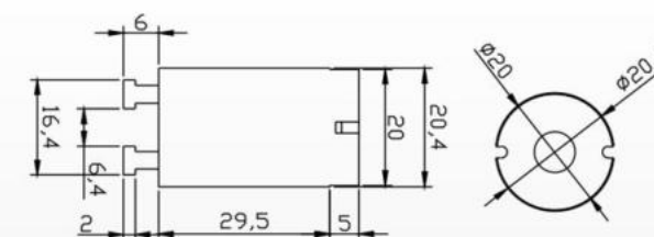
S-4 Material: PP Packing: 1000pcs/ctn G.W: 4.7kgs Ctn Size: 44X23X22cm
