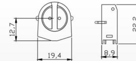
HD-2(G5) Material: PC Packing:4400pcs/ctn G.W:11.4kgs Ctn Size: 38X28X30cm
