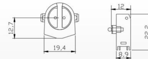
HD-2A(G5) Material: PC Packing:4400pcs/ctn G.W:12.7kgs Ctn Size: 38X28X30 cm
