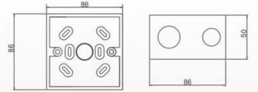
HS-86x86x50 Material:PVC
