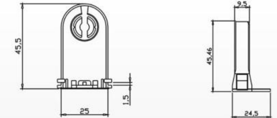
HB-33B(G13) Material: ABS PC Packing: 1400pcs/ctn G.W: 10.1kgs Ctn Size: 38X28X30cm
