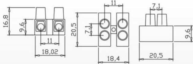
H-10A(10mm 2 ) (2P,3P,4P)
