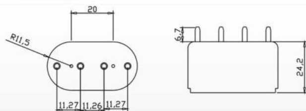
HE-3(2G11) Material: PBT Packing:1000pcs/ctn G.W:13kgs Ctn Size: 38X28X30cm
