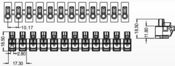
HA-25(2.5mm 2 ) (2P,3P,4P,12P)
