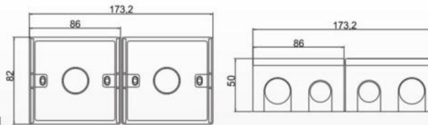
HS-86X86X50 Material:PVC Packing:200pcs/ctns Ctn size:43x35x51cm Color:White Grey Red
