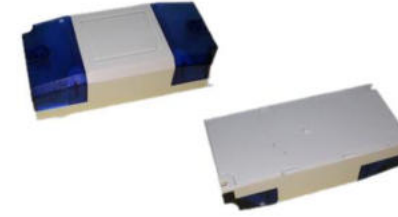
LED-02 (94x45x28mm) Material: PC
