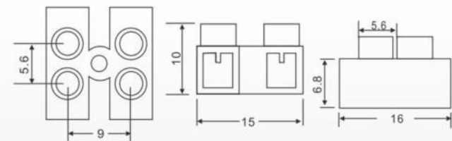
HA-40 (H-2.5A,2.5mm 2 ) (2P,3P,4P)
