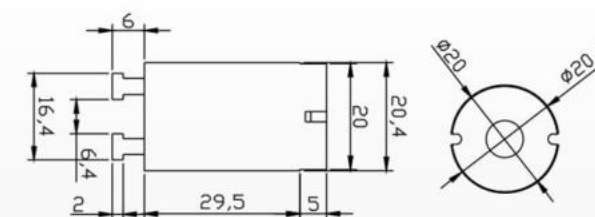
S-3 Material: PP Packing: 1000pcs/ctn G.W: 4.7kgs Ctn Size: 44X23X22cm
