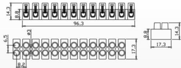
JP-PA7-F(12P) (17.5A,450V) Flat Base Material: PA,Steel Insert
