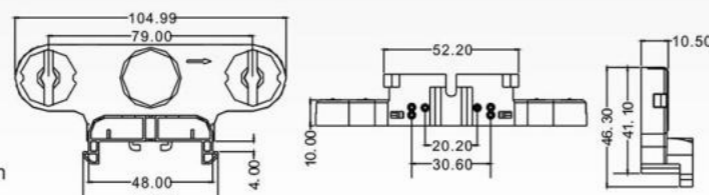
HB-38F(G13) Push-out & electron type
