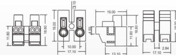
HA-25A(2.5mm 2 ) (2P)
