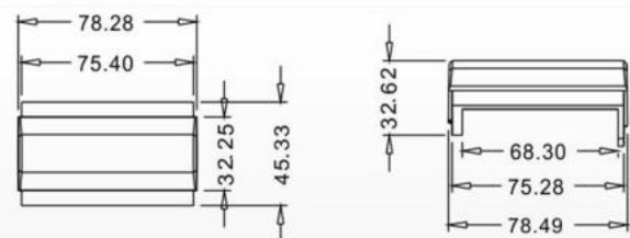
H-27 Material: ABS Packing: 300pcs/ctn G.W: 8.5kgs Ctn Size: 38X28X30cm
